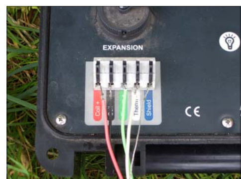
Typical readout panel and connections
